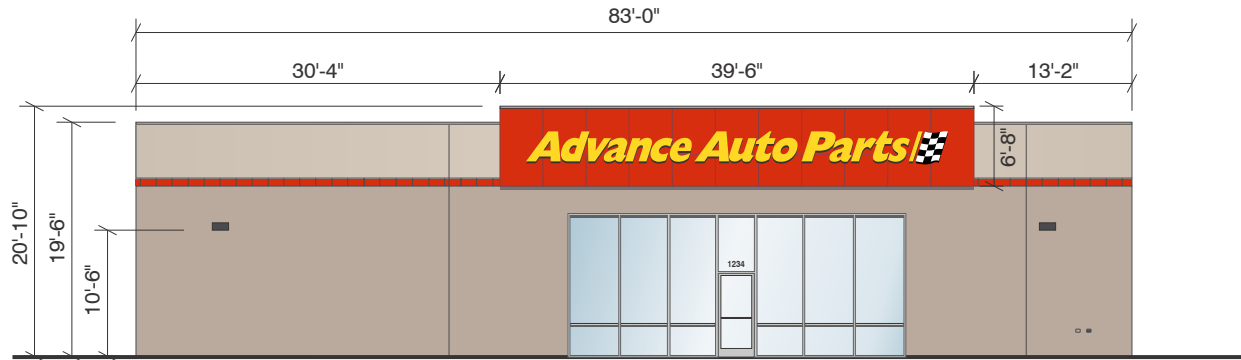
FRONT ELEVATION Scale: 1/16" = 1'-0"
